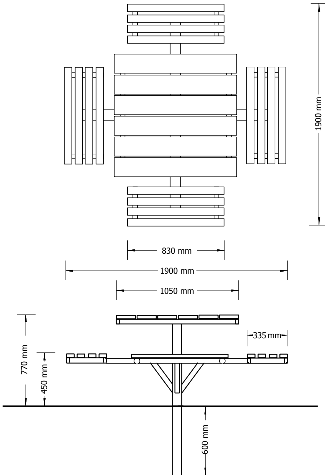
Side elevation
